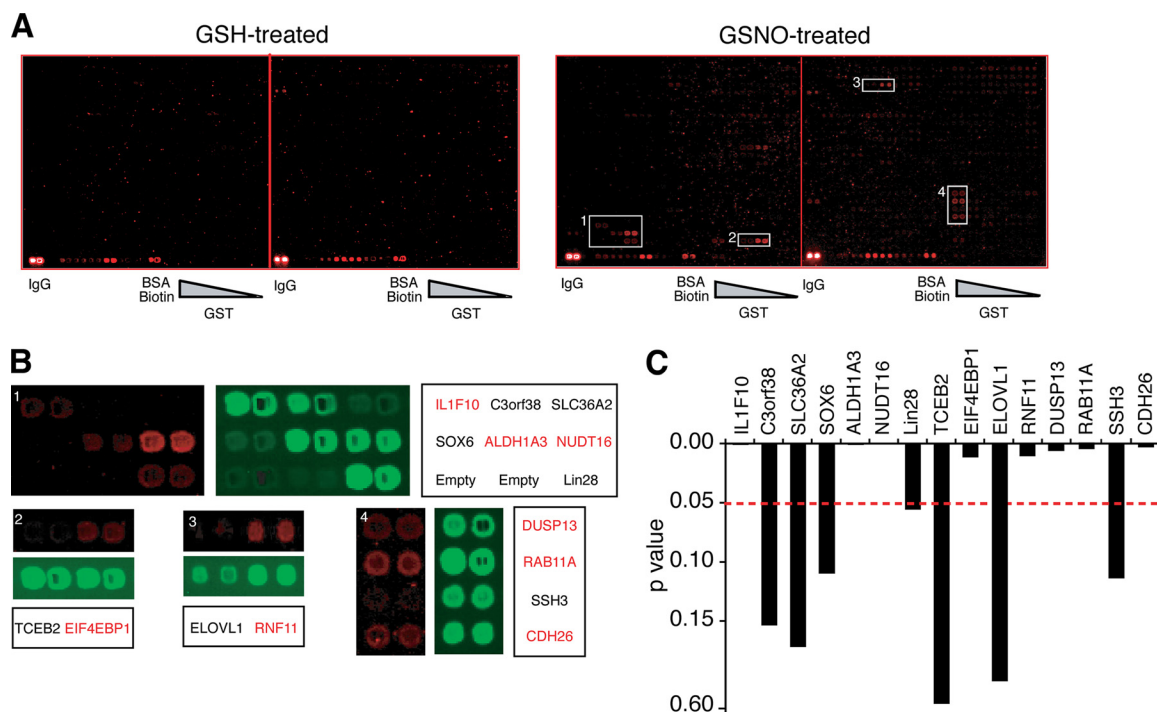
FIG. 2. Detection of S-nitrosylated proteins on the human proteome chip. A, Cy5 fluorescence of two representative blocks (#26 and #27 of 48) of the protein chip treated with GSH (100 \mu M, 1 h) or GSNO (100 \mu M, 1 h). IgG and biotin labeled bovine serum albumin (BSA-biotin) serve as positive controls. A gradient of GST at the bottom right of chip serves as a GST control. White rectangles indicate magnification area for (B). B, Magnified images of proteins identified as S-nitrosylated are shown in red. C, The p values of the 15 proteins shown in (B). All experiments were repeated three times.
