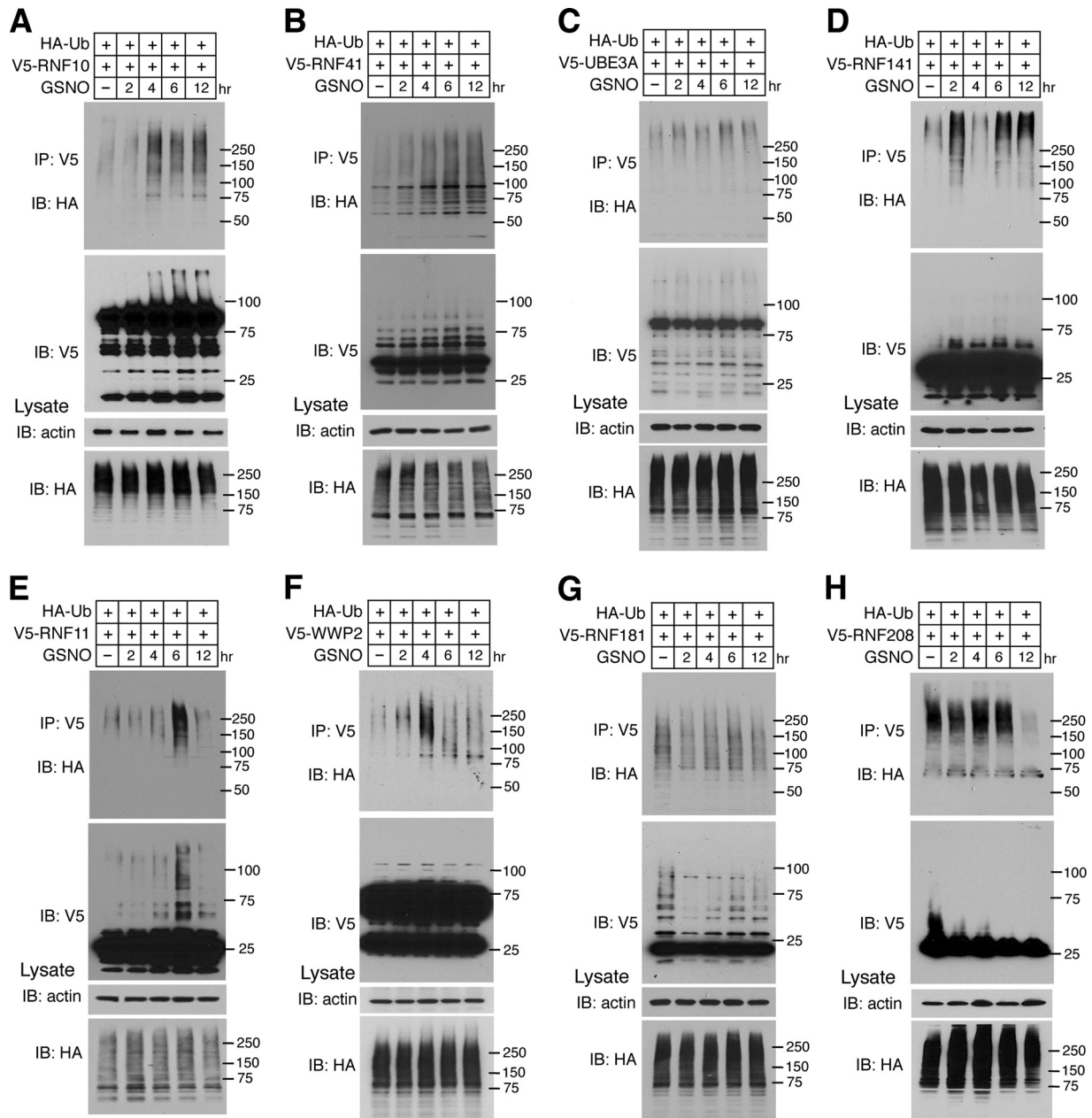
FIG. 5. Ubiquitin E3 ligase activity of A , RNF10, B , RNF41, C , UBE3A, D , RNF141, E , RNF11, F , WWP2, G , RNF181, and H , RNF208 was analyzed by an in vivo ubiquitination activity assay with or without GSNO treatment for 0, 2, 4, 6, and 12 h.
